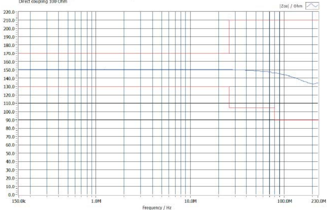
Typical common mode impedance
