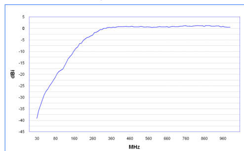
Gain Diagram BicoLOG 30100
