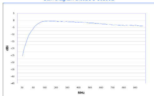
Gain Diagram BicoLOG 30100E
