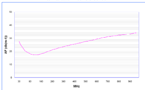
Antenna factor BicoLOG 30100E
