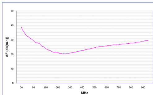
Antenna factor BicoLOG 30100
