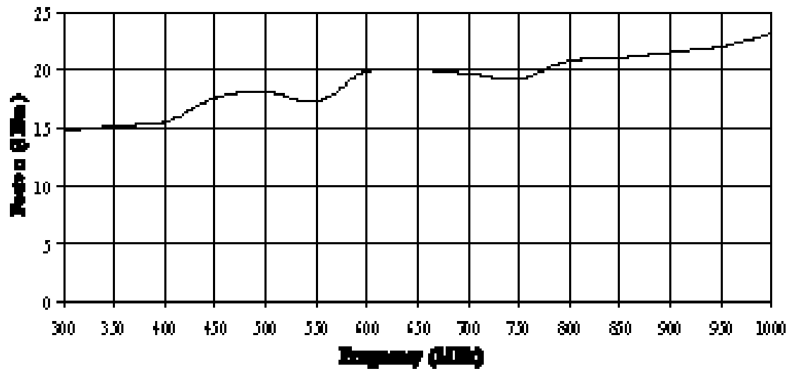
Figure 1.2 - Typical Antenna Factors for AL-100 Log Periodic Antenna
