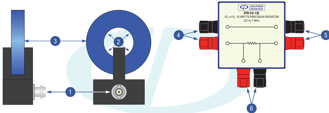
FIGURE 2 - AL-RS101-RX Features
