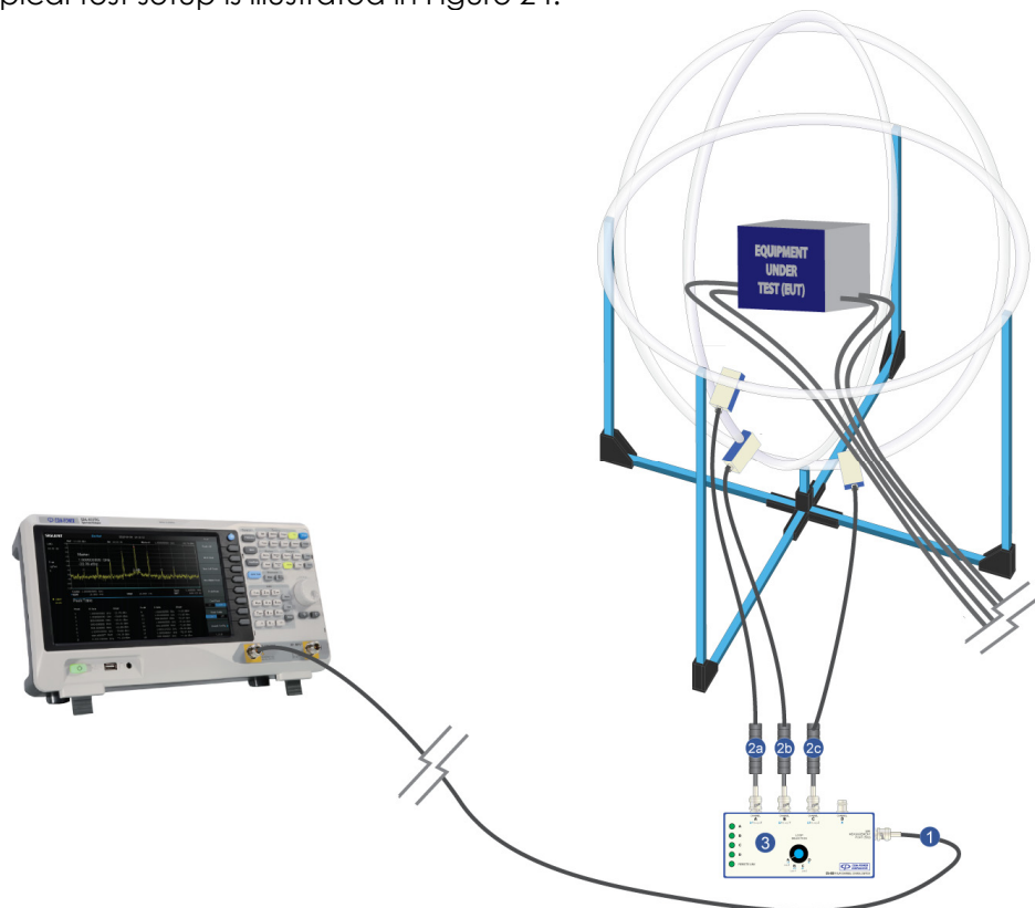
Figure 24 - Typical Test Setup for Disturbance Measurements
