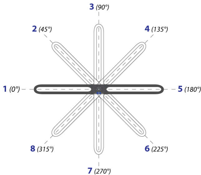
Figure 26 - Balun-Dipole Positions During Calibration
