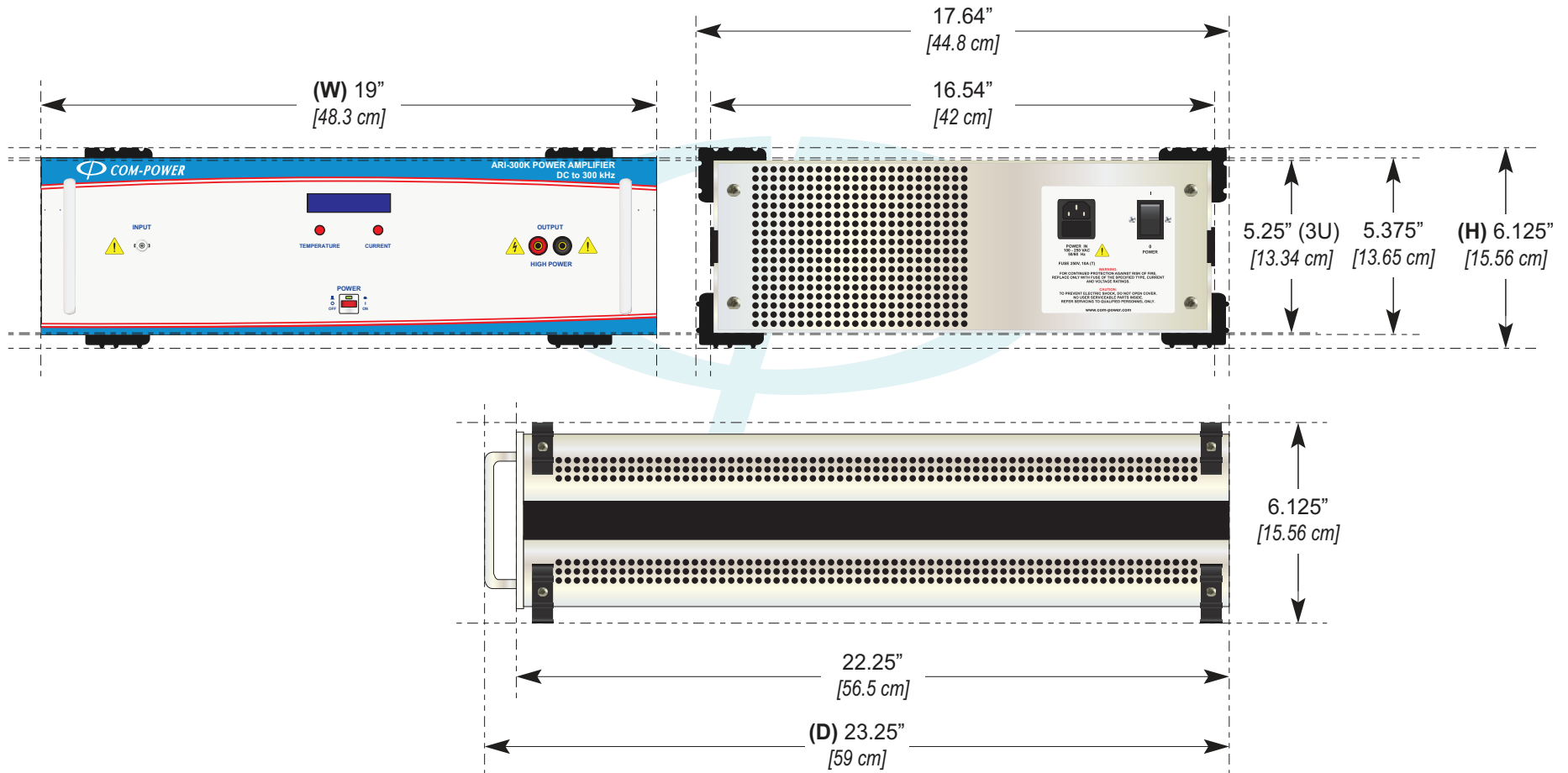
FIGURE 3 - Product Dimensions
