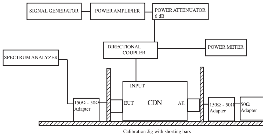
Figure 2-5 Level measurement setup using CDN
