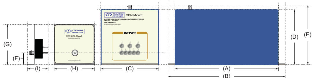
Figure 2 - Product Dimensions
