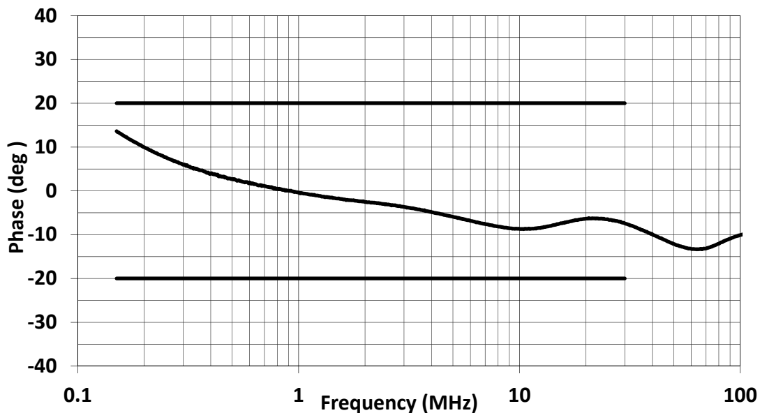
Figure 4 - Phase compared to CISPR 16-1-2 edition 1.2 requirements.
