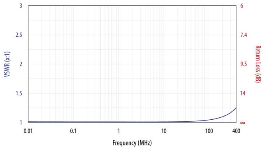
Figure 6 – Typical VSWR/Return Loss for FCLCE-1000 Calibration Fixture
