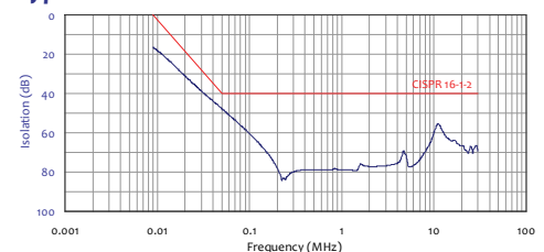
Typical Isolation Data
