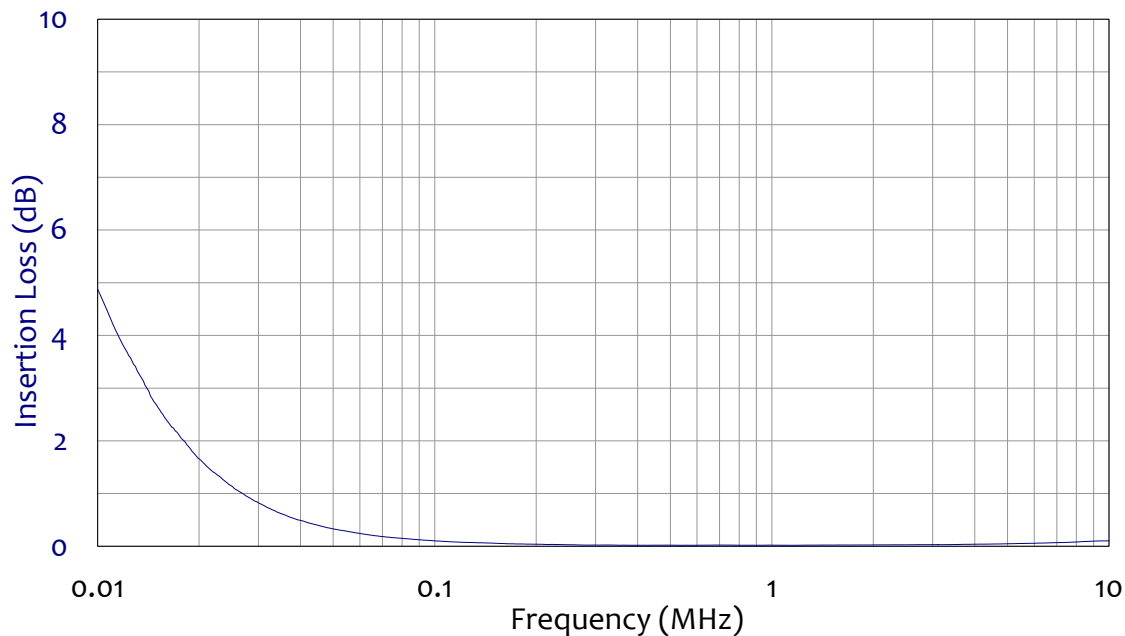
Figure 3 – Insertion Loss
