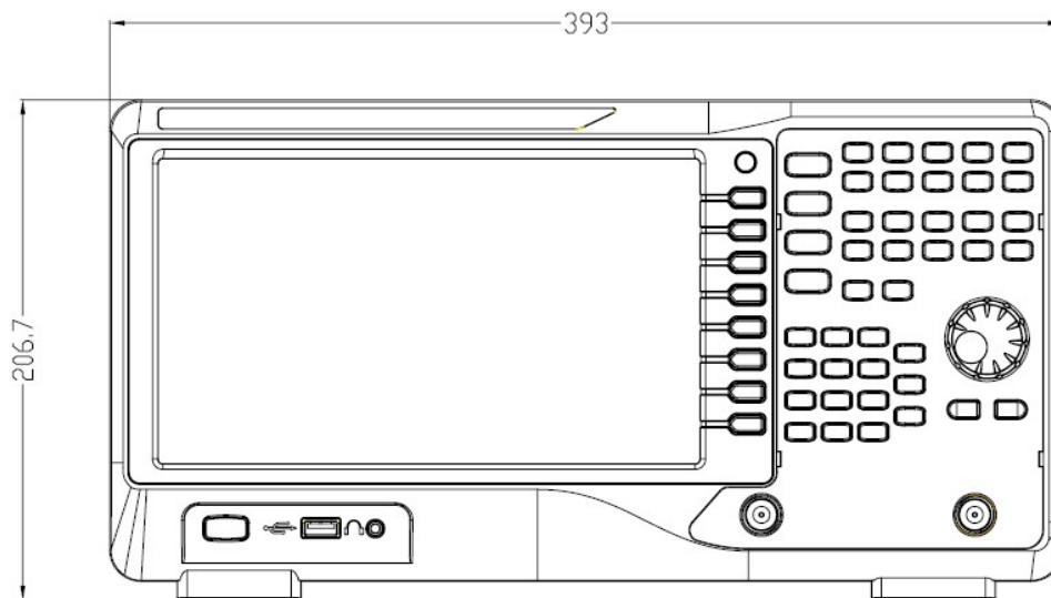
Figure 1-1 Front View
