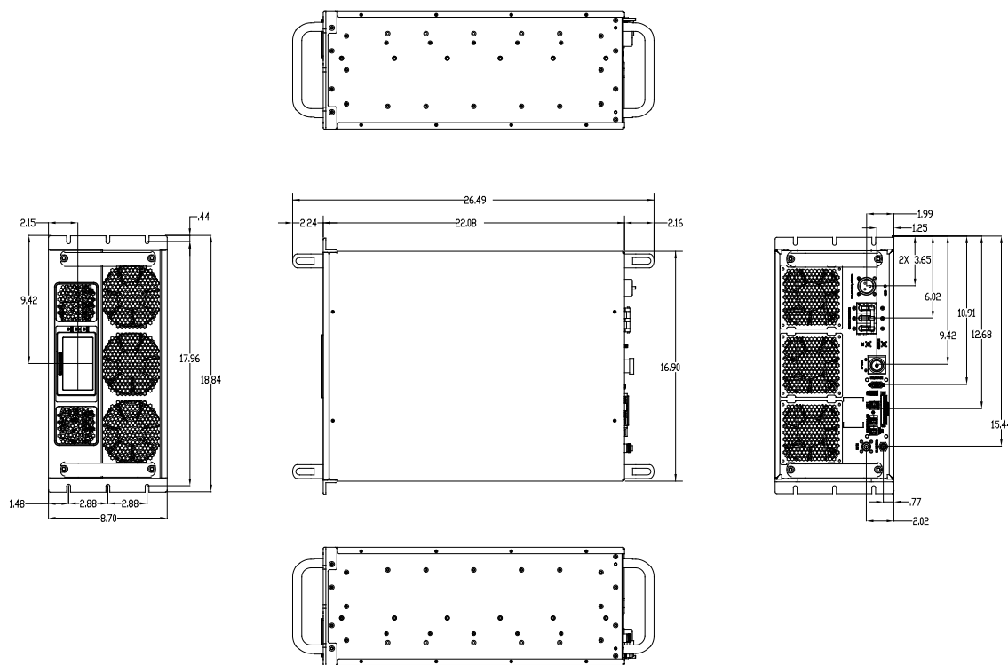
2199-00X – Front and Rear View
