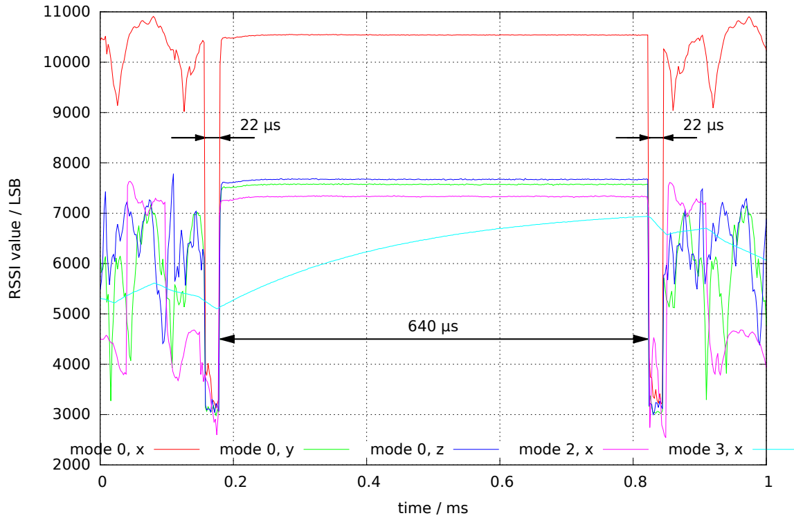
Figure 8: Close-up of periodic breaks of the jamming pattern, synchronized with the break
