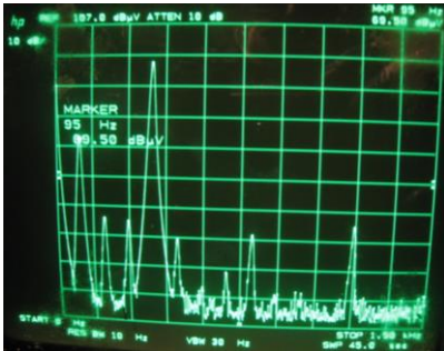
Figure 4a: View of 6.3 Vrms 100 Hz ripple on a 400 Hz 115 Vrms bus, using the PRD-120
