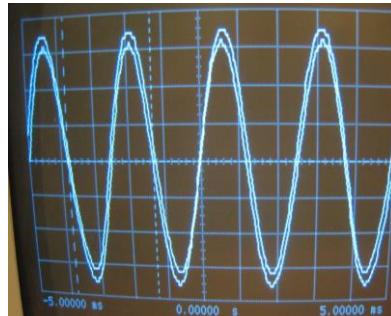
Figure 4b: Envelope of the same 100 Hz ripple on the same bus, using an oscilloscope
