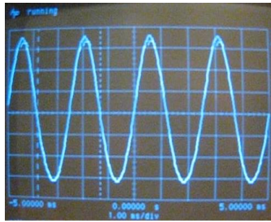
Figure 3b: View of the same ripple on the same bus, using an oscilloscope
