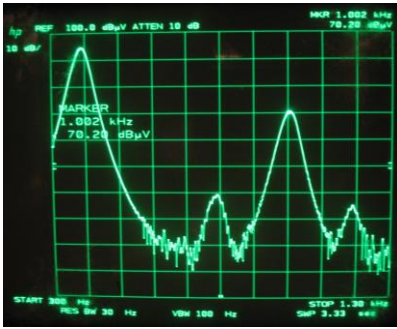
Figure 5a: 1 kHz ripple in span to 1300 Hz
