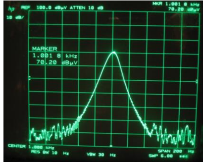
Figure 5b: 1 kHz ripple at center of 100 Hz span
