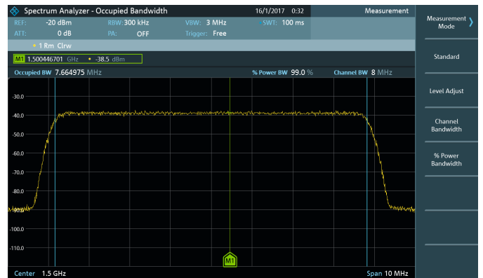
R&S®FPC-K55: occupied bandwidth measurement
