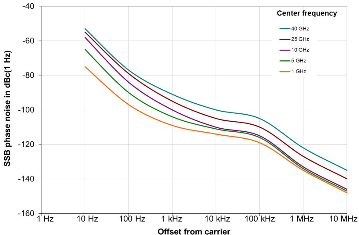
Typical phase noise at different center frequencies
