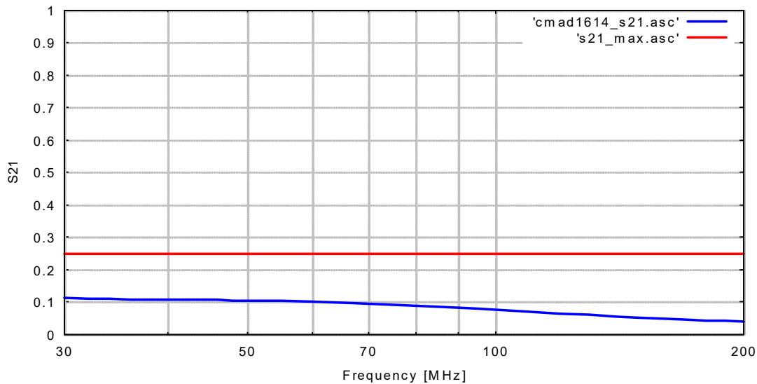
S21 measured acc. CISPR 16-1-4 Section 9.6
