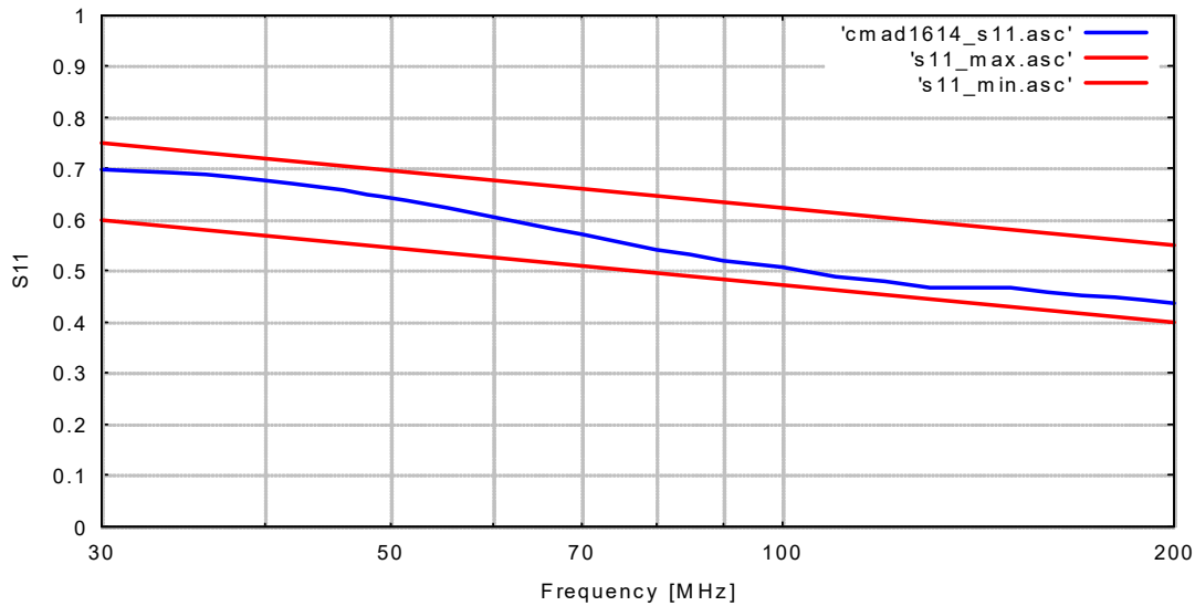
S11 measured acc. CISPR 16-1-4 Section 9.5
