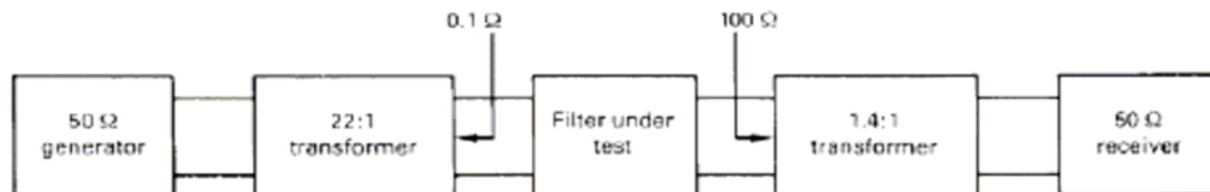
Figure C.1 — Test circuit
