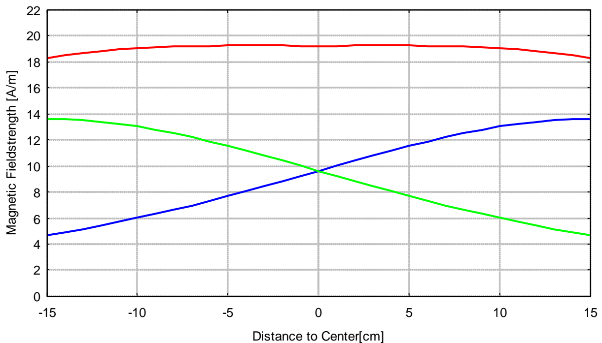
HHS 5206-8 magnetic Fieldstrength along longitudinal coil axis
