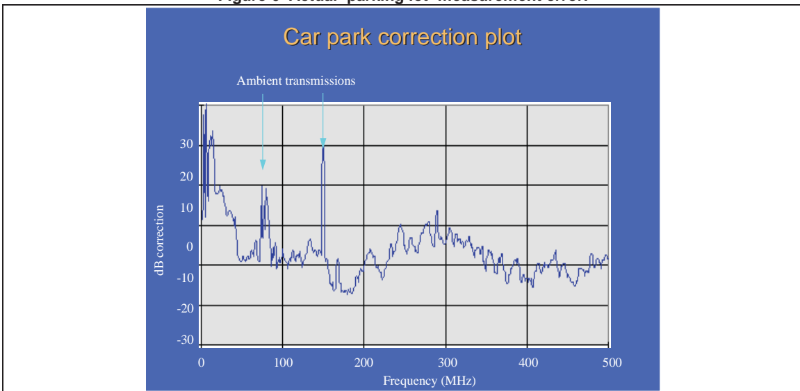
Figure 6 Actual 'parking lot' measurement error.
