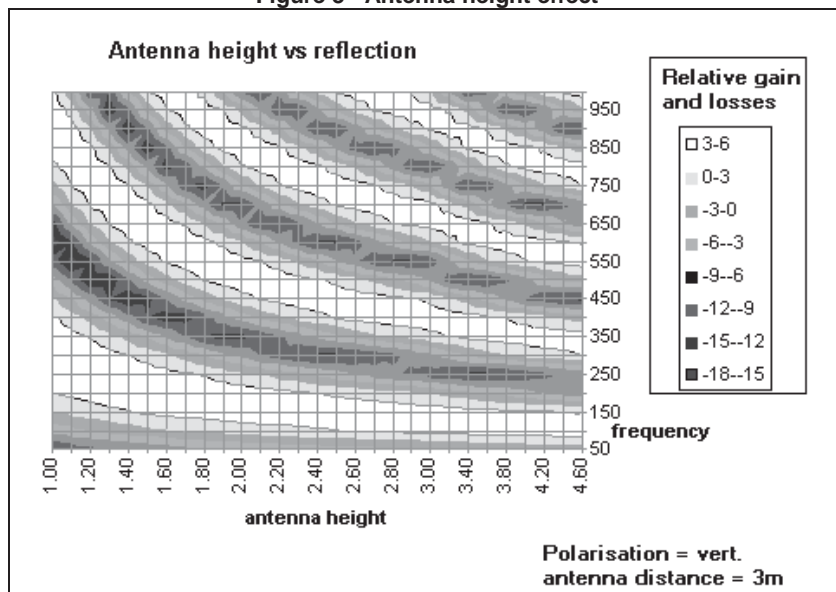
Figure 3 Antenna height effect
