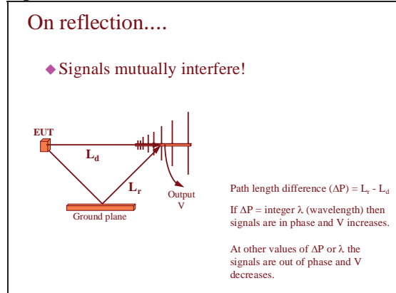
Figure 2 The reflection mechanism
